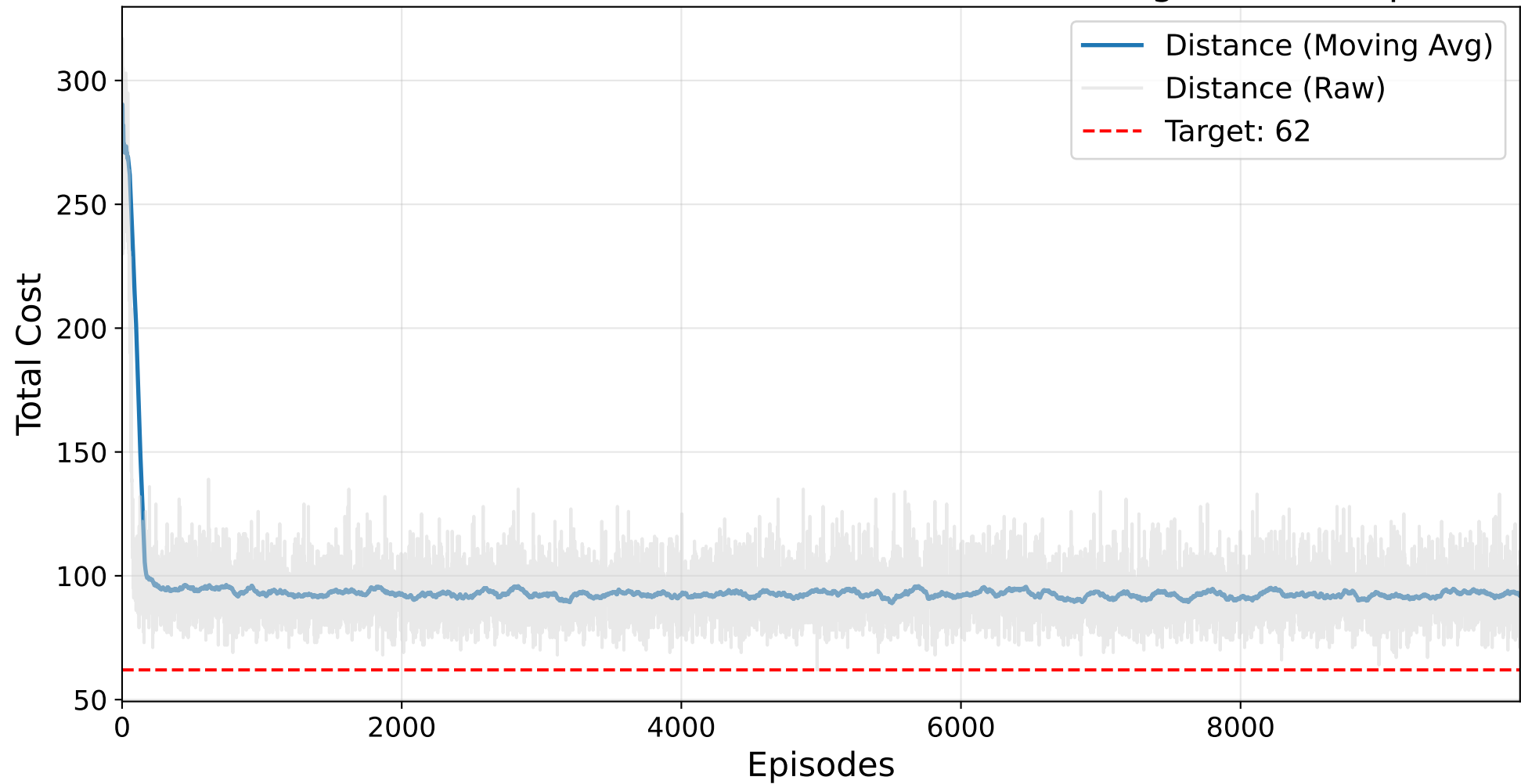
Final HYPERBAND GP Masked AutoRL-SOP Training - ESC63.sop
